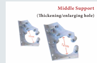
50/70/100 N motor (100) (50/70)
