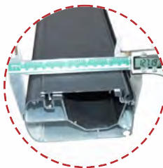
Front tube, width 127mm
